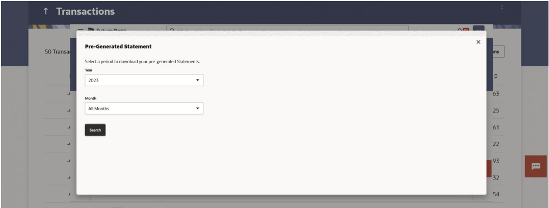
Figure 6-5 Pre-generated Statement
