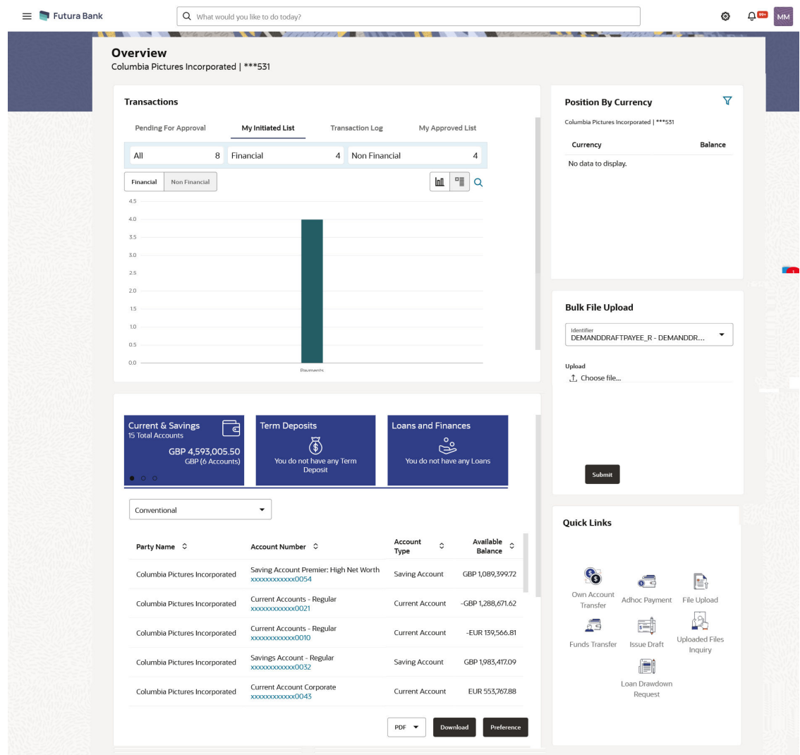
Figure 1-1 Overview widget
